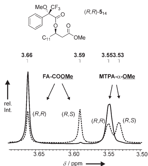
Figure 2. ^1\text{H} NMR (400 MHz, \text{CDCl}_3 , OMe area, \delta = 3.7\text{--}3.5 ppm) of MTPA derivative 5 14 . The MTPA ester obtained from racemic methyl 3-hydroxymyristate ( rac - 4 14 ) shows signals for both the ( R,S ) and the ( R,R ) diastereomers (dotted line). The corresponding Mosher's ester derivative ( R,R )- 5 14 obtained by asymmetric ( R )-BINAP- \text{RuCl}_2 -catalyzed hydrogenation shows only one set of signals, allowing the determination of optical purities by integration (98.3% dr in ( R,R )- 5 14 , corresponding to 98.3% er in ( R )- 4 14 ).
